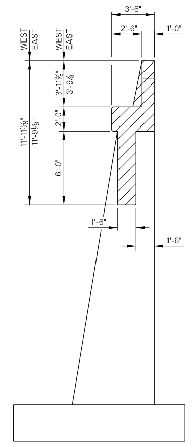
TYPICAL SECTION
